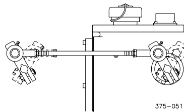
Figure 1. Linear Linkage
